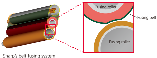
Sharp's belt fusing system
